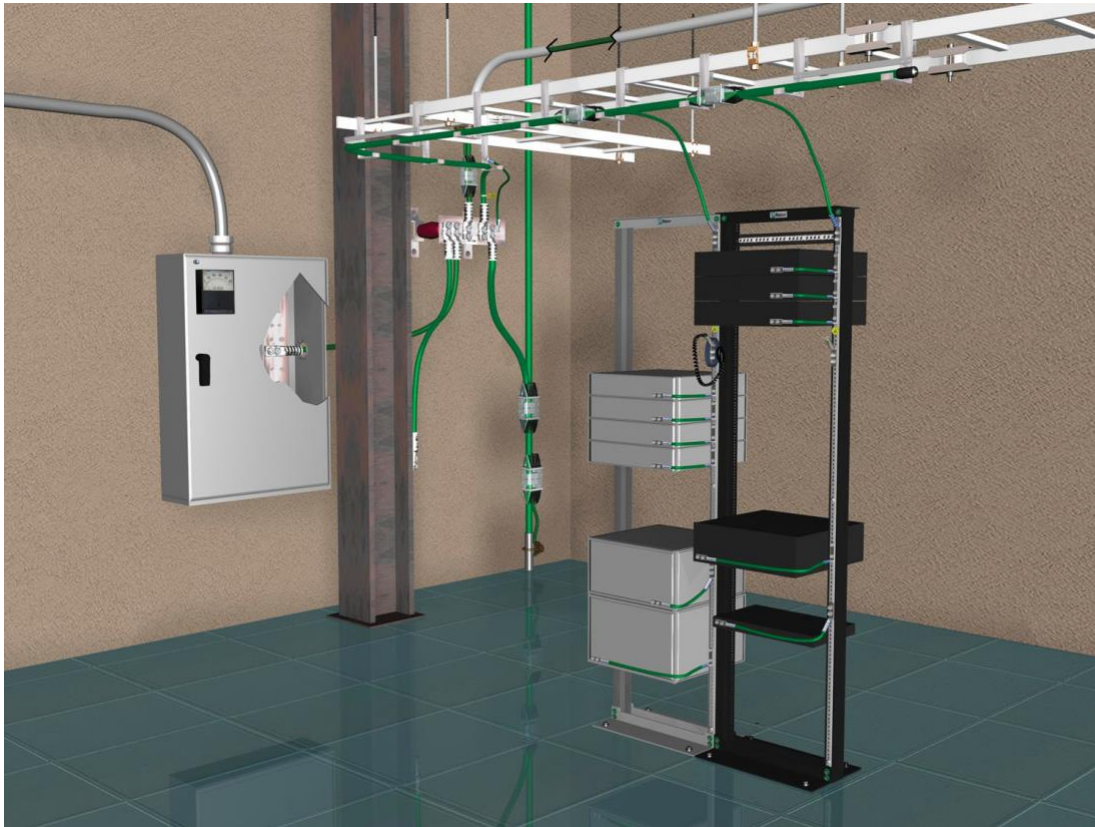
Figure 5: Grounding and Bonding in Telecommunications Room
