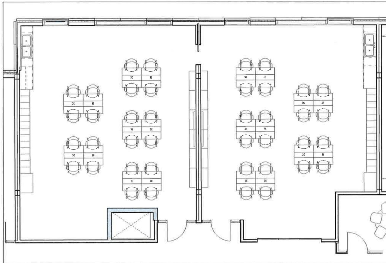
GRADES 2-5 LEARNING COMMUNITY - CLASSROOM PLAN
