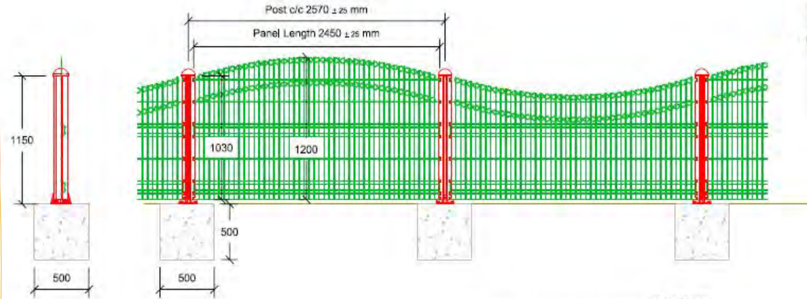
120x100 mm K-DAG ALUMINIUM ILLUMINATED FENCE POST
