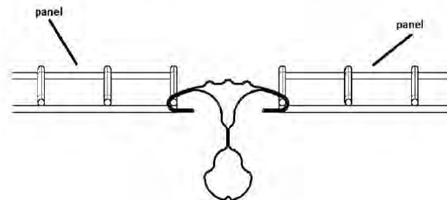
BEAR GRIP SELF-LOCK POST WITH SOLAR LIGHT POST CAP
