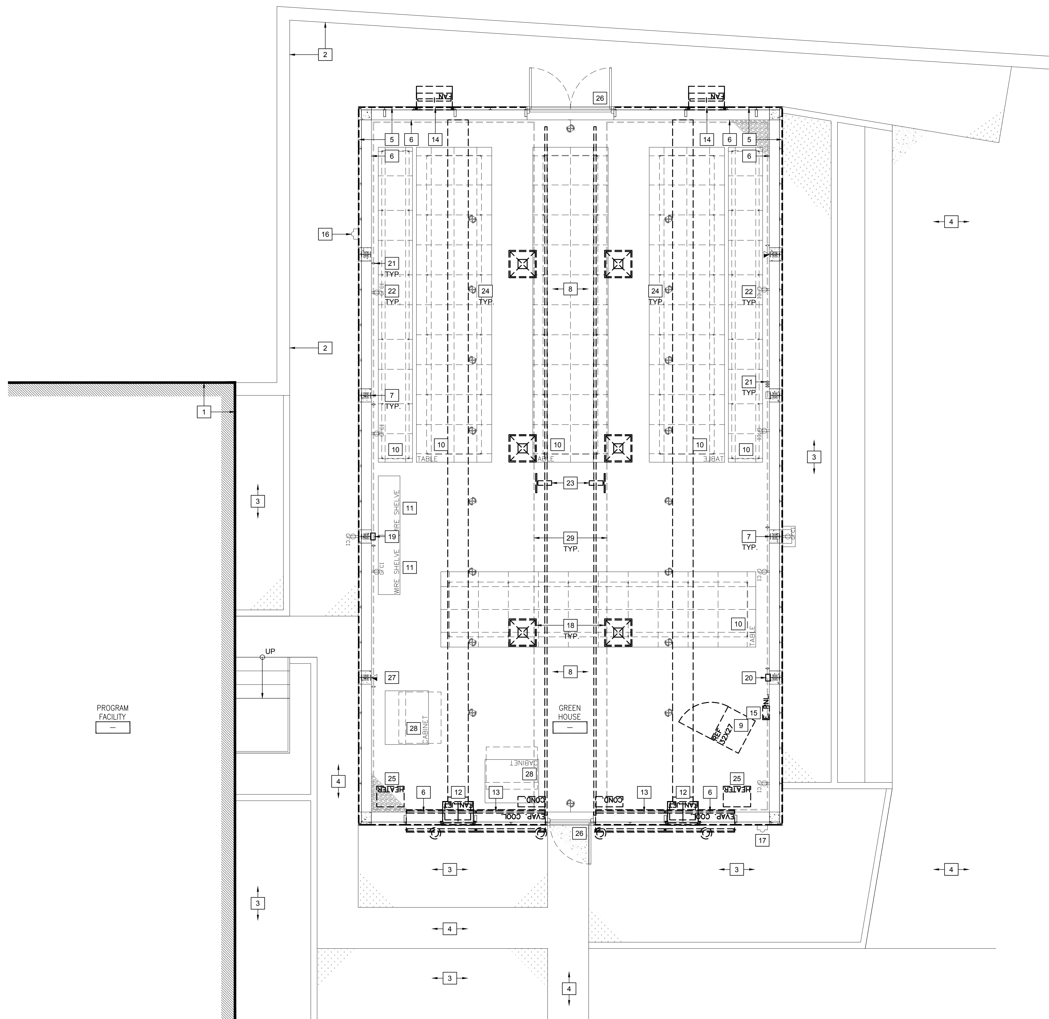
1 DESIGN BUILD SCOPE PLAN SCALE: 1/4" = 1'-0" ARCHITECTURAL
