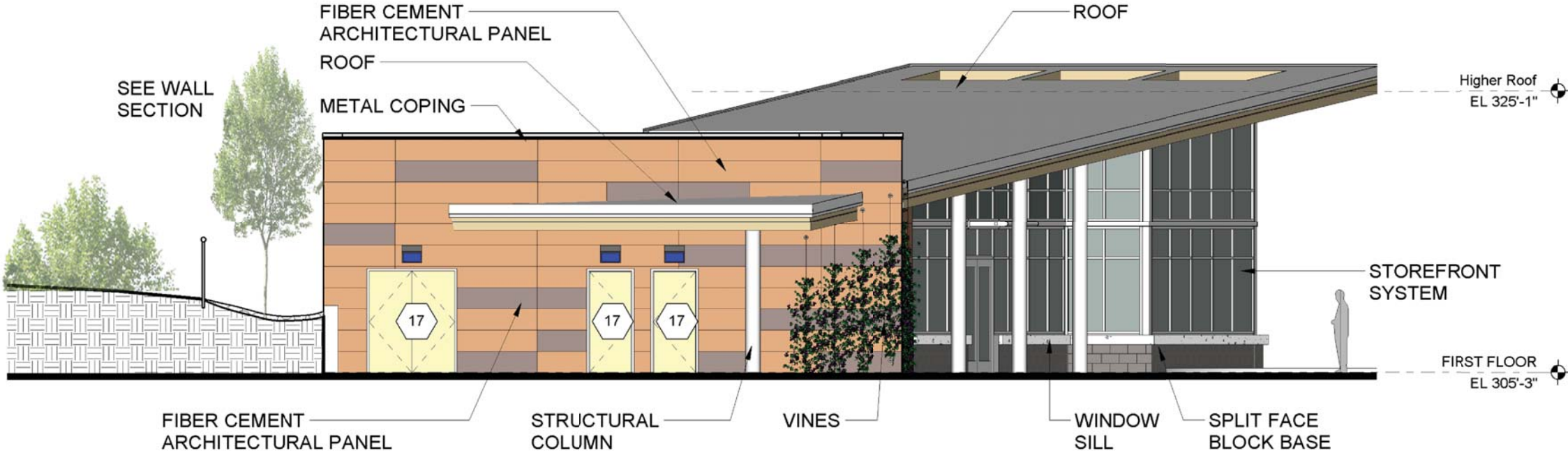
NORTH ELEVATION
