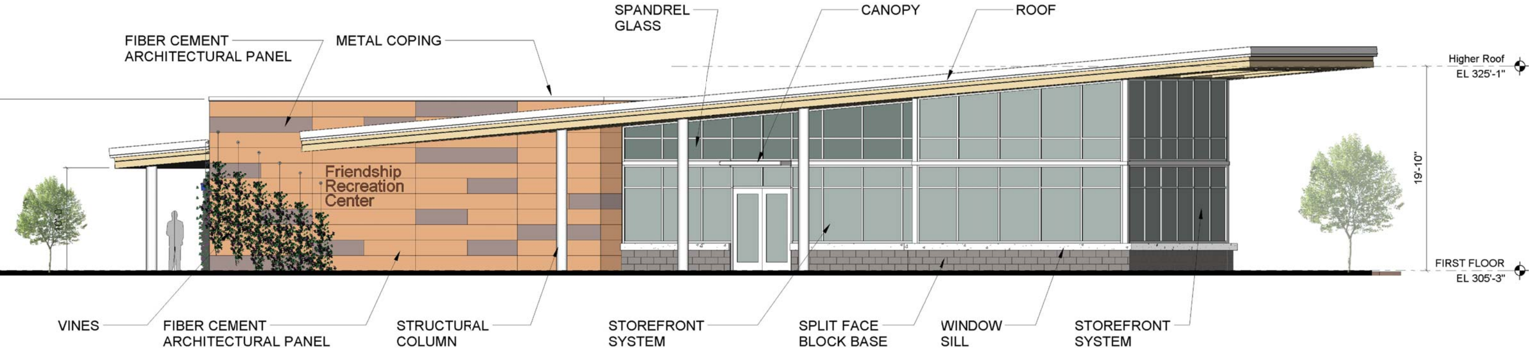
WEST ELEVATION
