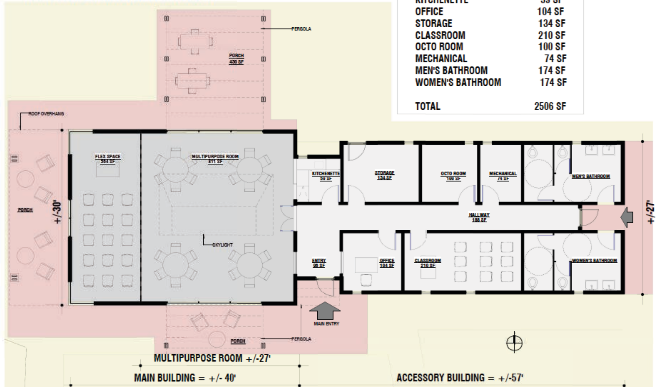
FLOOR PLAN AND SQUARE FOOTAGE ALLOCATION
