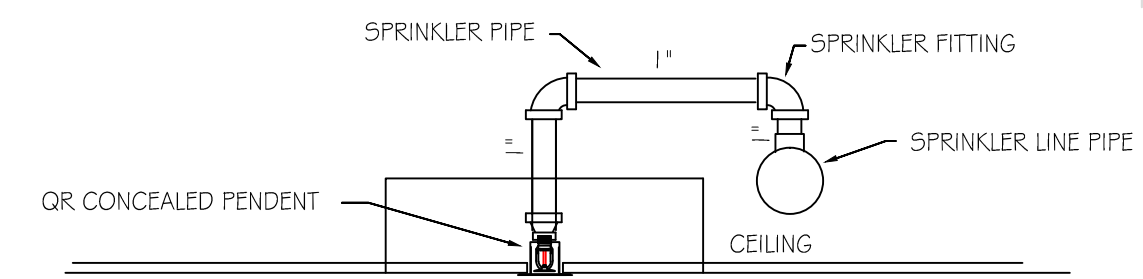
RETURN BEND DETAIL (GOOSENECK) SCALE: NONE
