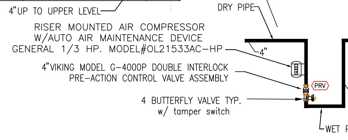
PREACTION SYSTEM SECTION SCALE: NONE
