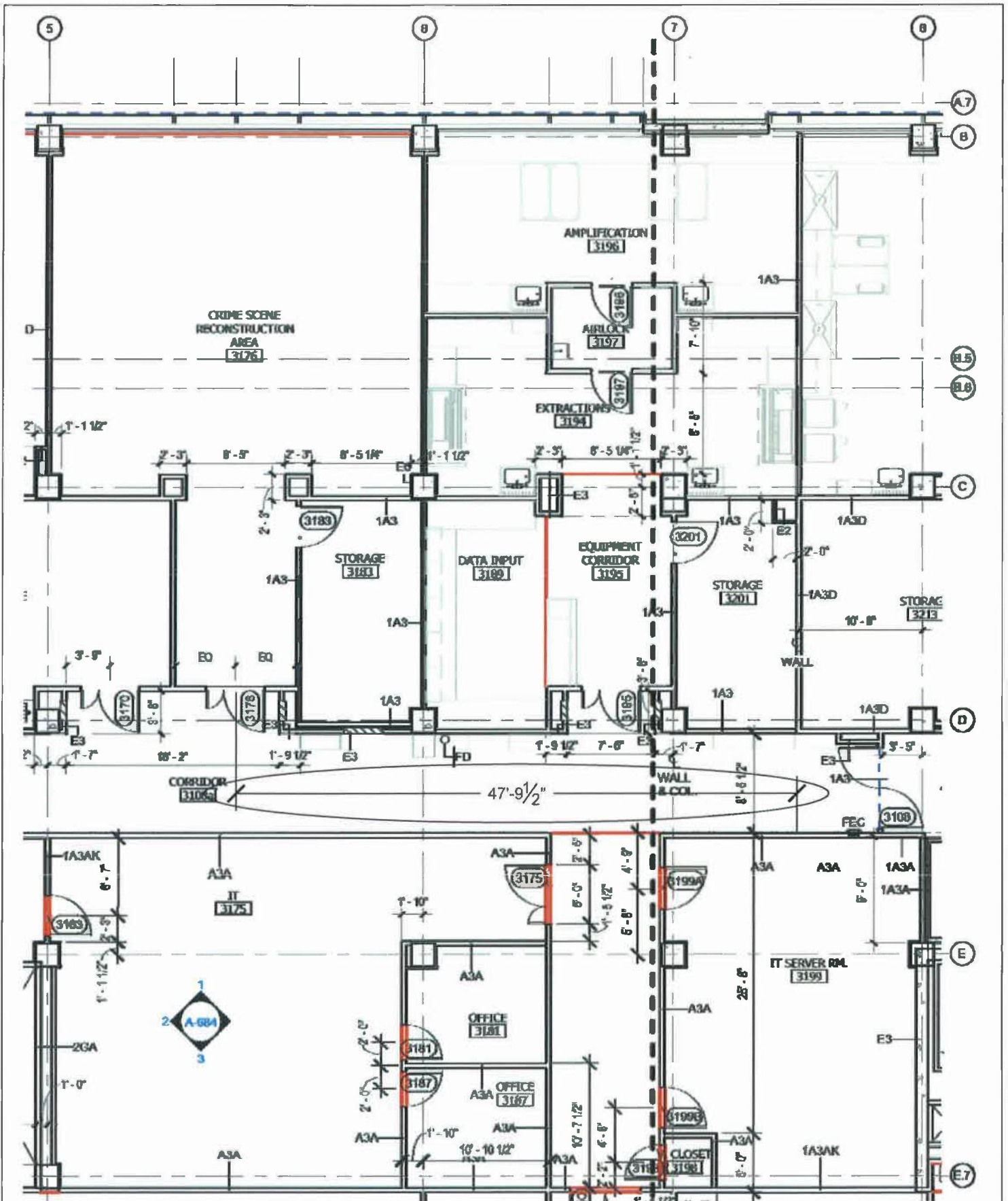
ATTACHMENT A-7 PARTIAL FLOOR PLAN SCALE: 1" = 3/32"
