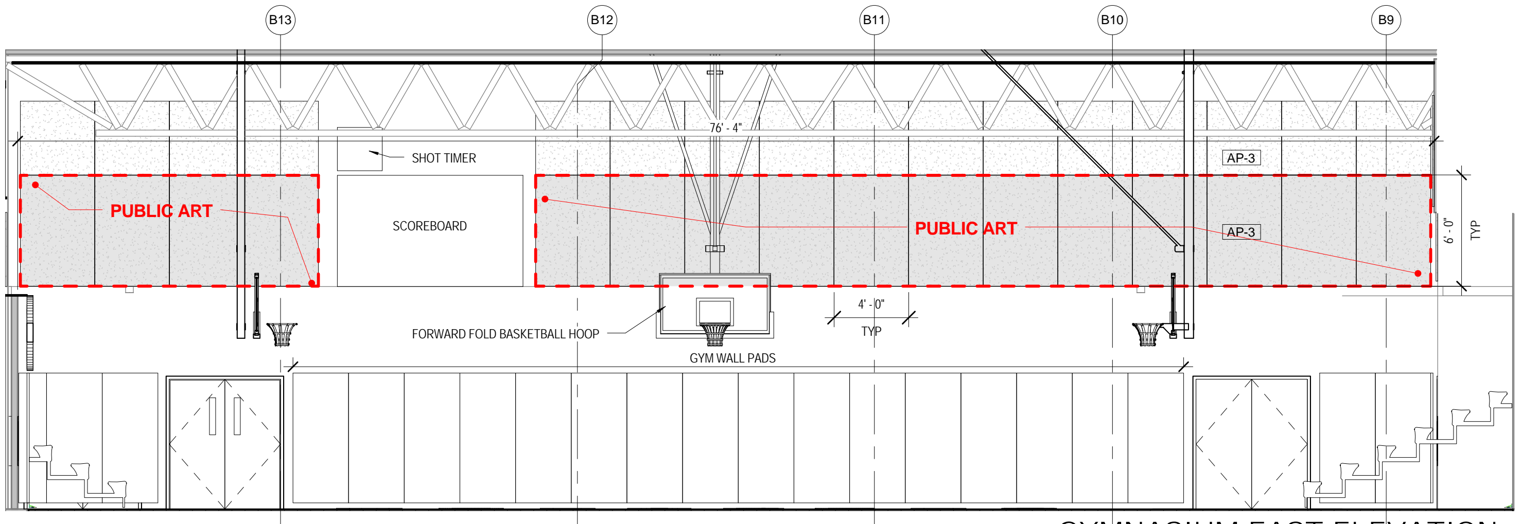
GYMNASIUM EAST ELEVATION WEST ELEVATION SIMILAR
