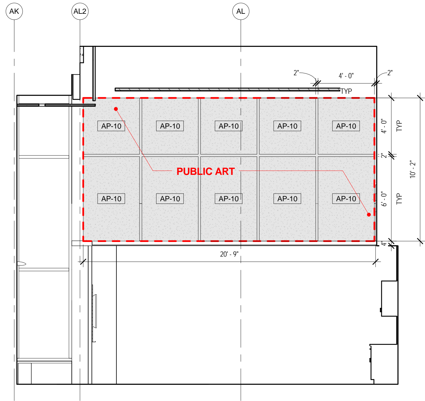
LIBRARY SOUTH WALL ELEVATION. NORTH WALL ELEVATION SIMILAR
