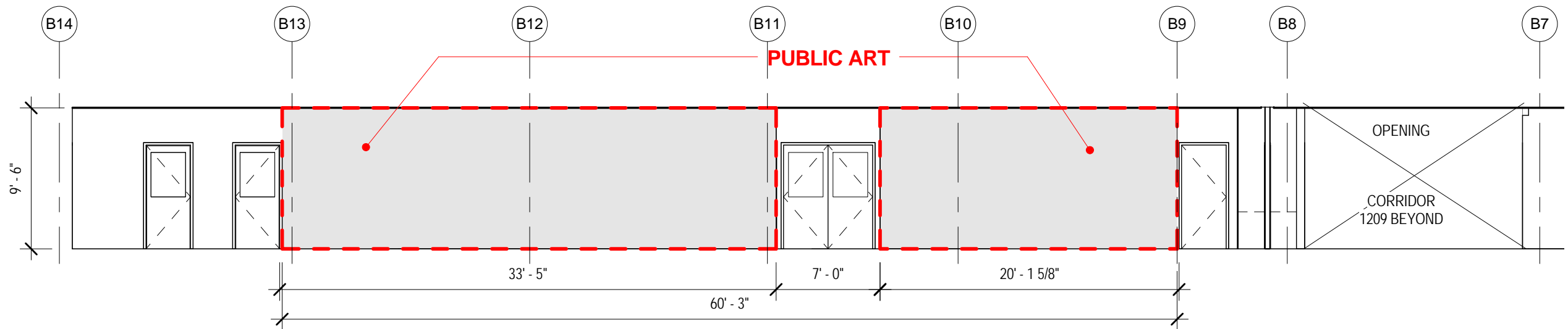
FRATERNITY HALL - EAST ELEVATION
